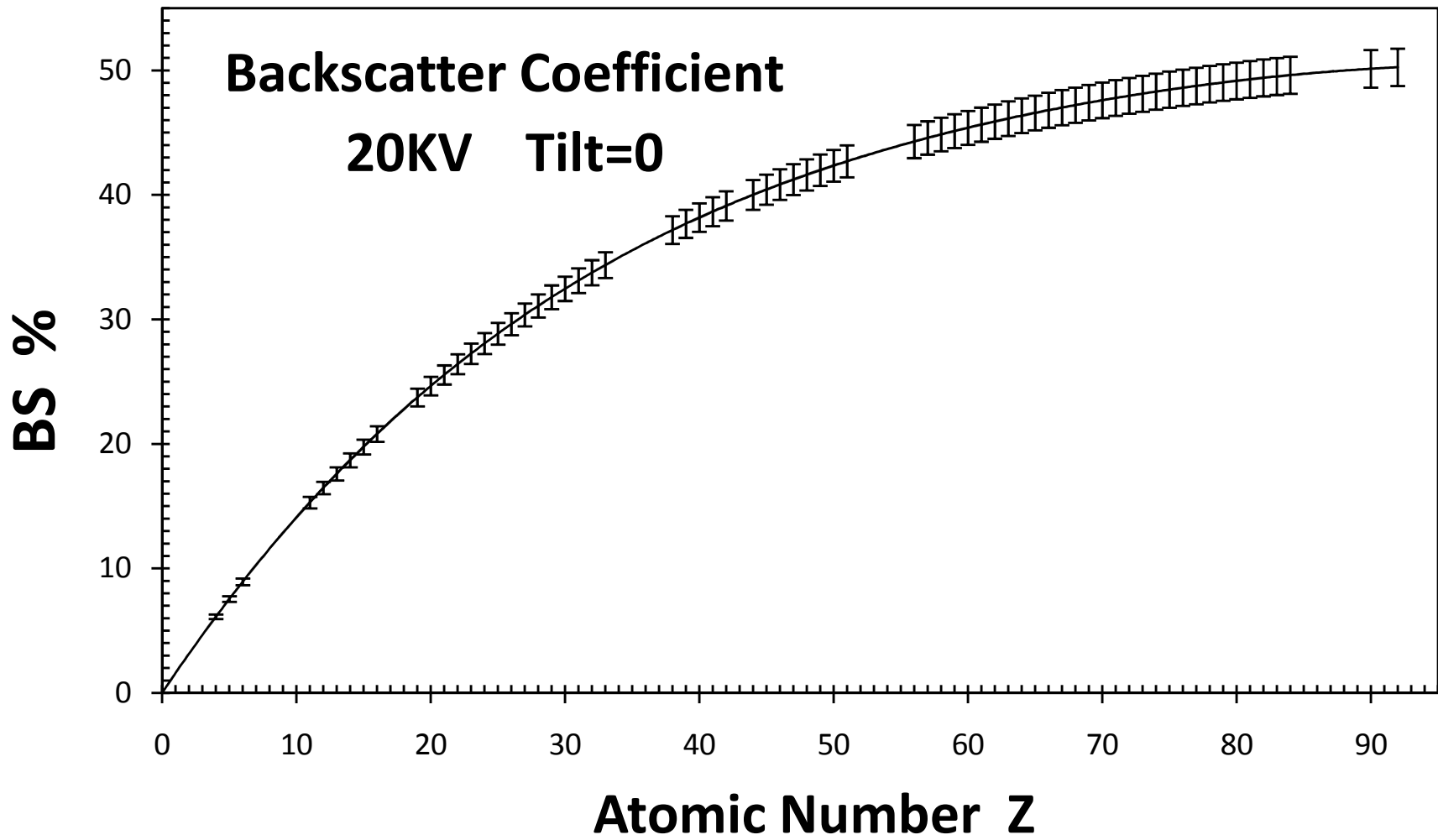
Figure 1. The calculated electron backscatter coefficient, using 20KV and no tilt.
