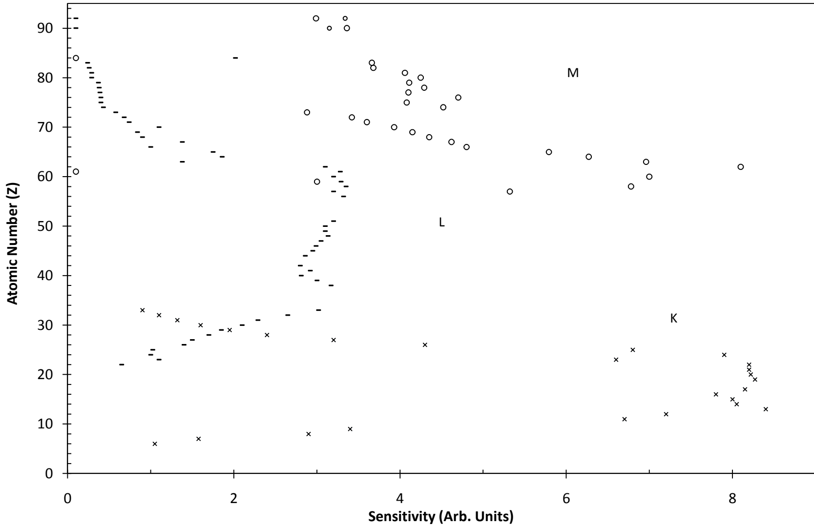
Figure 1. The peak sensitivity for the common elements, using EDS. Alpha K-peaks are indicated. Of the many L and M peaks, only the main peak is shown. Fitting this data would be very difficult, if not useless/inane.
