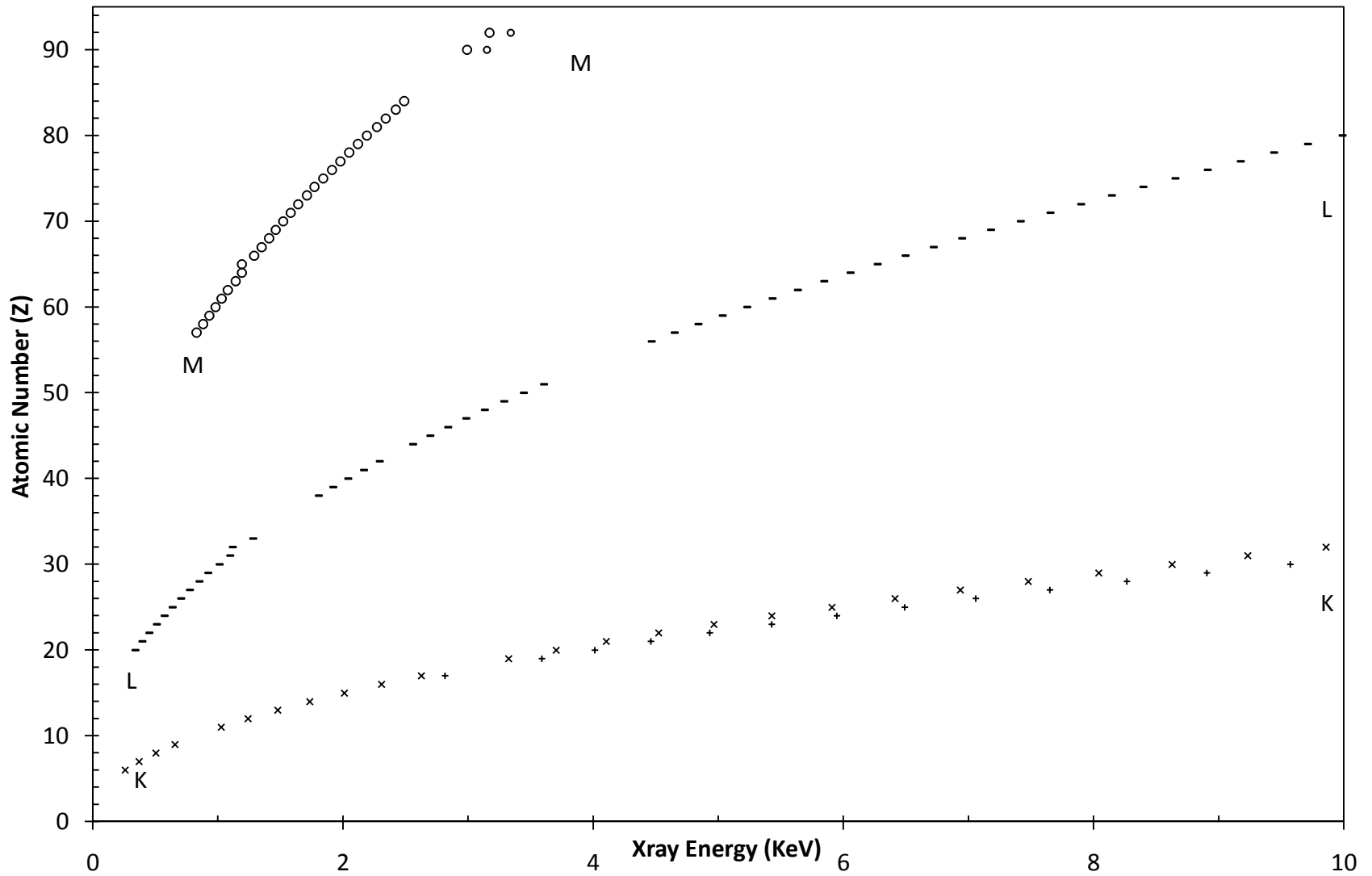
Figure 1. The peak energies for the common elements, using EDS. Both K-peaks are indicated, when significantly separated. Of the many L and M peaks, only the main peak is shown. Gaps are for rare and/or unseen elements.
